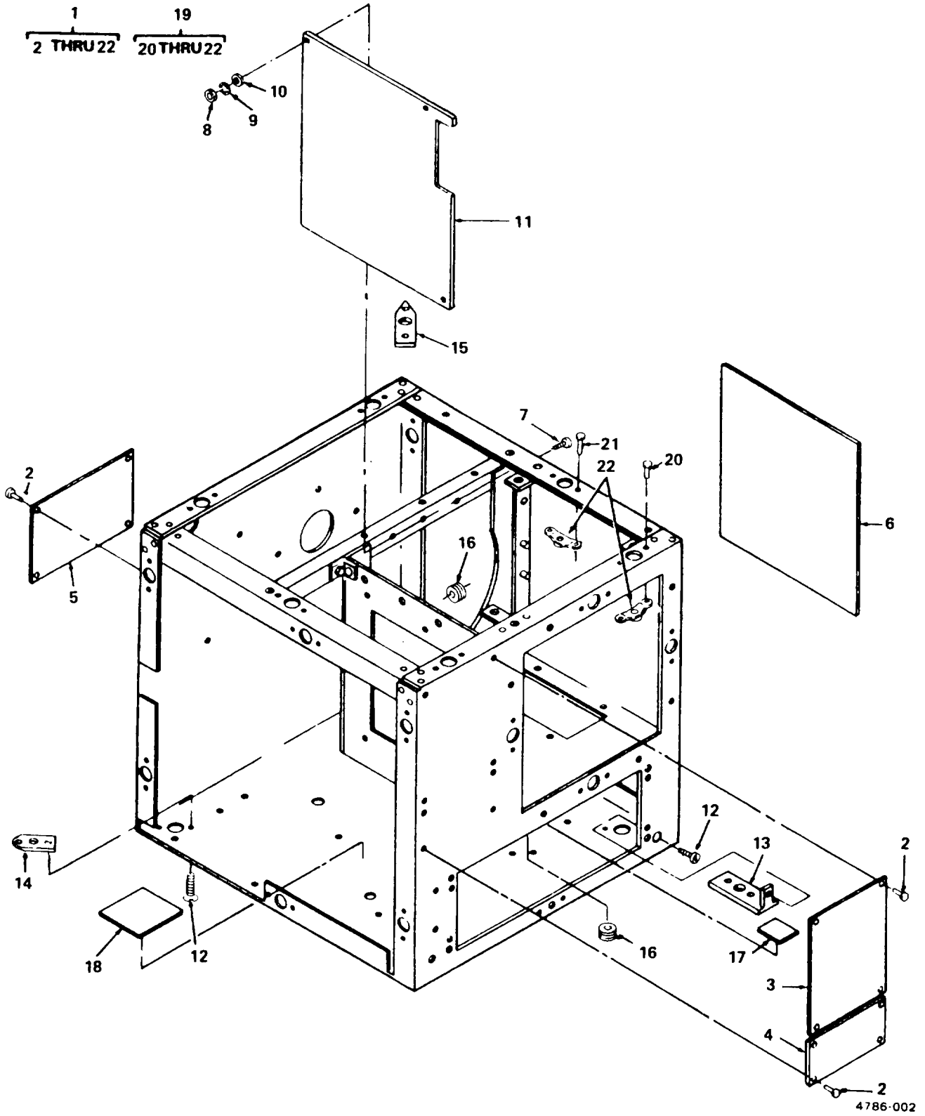
Figure 2. Case Assembly.
