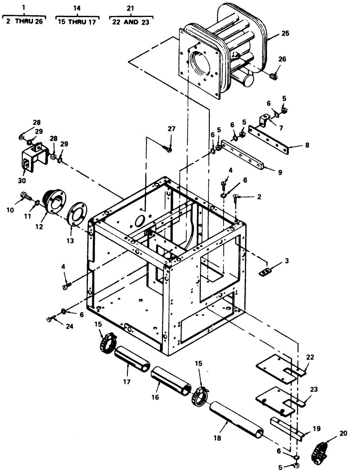
Figure 13. Heat Exchanger and Rainshield
